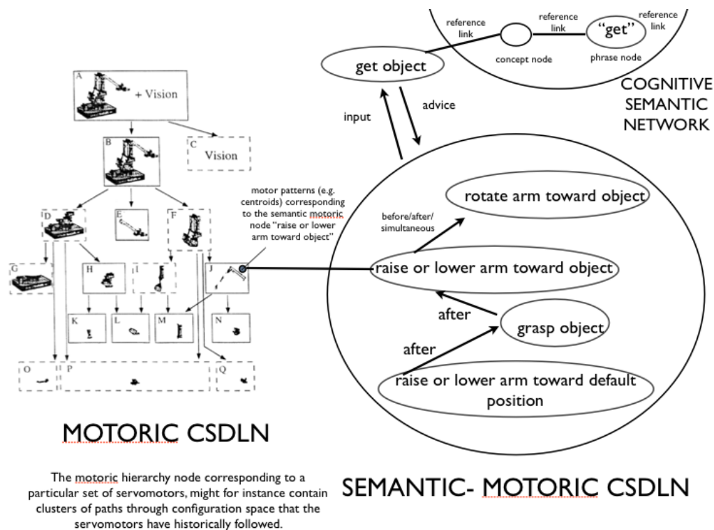
Figure 2: Simplified depiction of the relationship between a semantic-motoric CSDLN, a motor control hierarchy (illustrated by the hierarchy of servos associated with a robot arm), and a cognitive semantic network (like OpenCog's AtomSpace).
