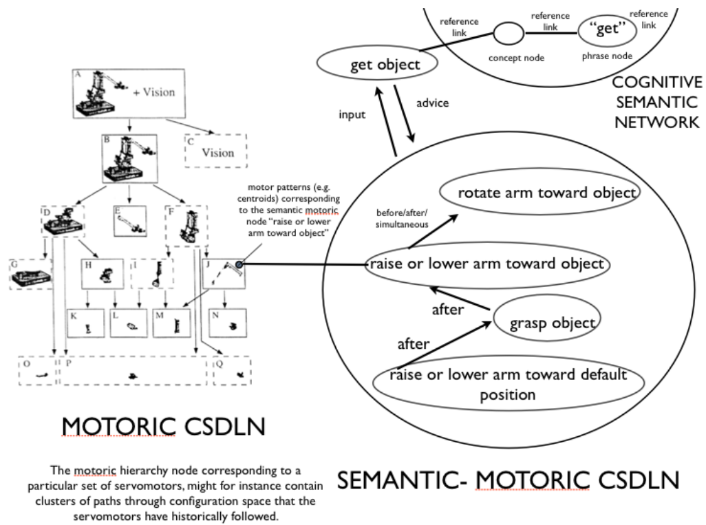
Figure 3: Simplified illustration of the proposed interoperation of perceptual, motoric and goal semantic CSDLNs.
